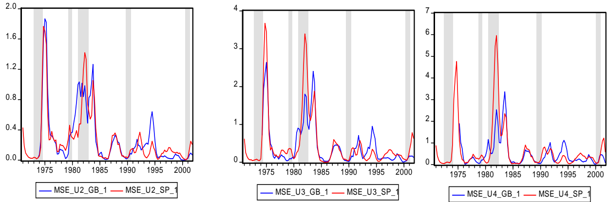
Figure 4: 1-Year Rolling MSE (Unemployment)
