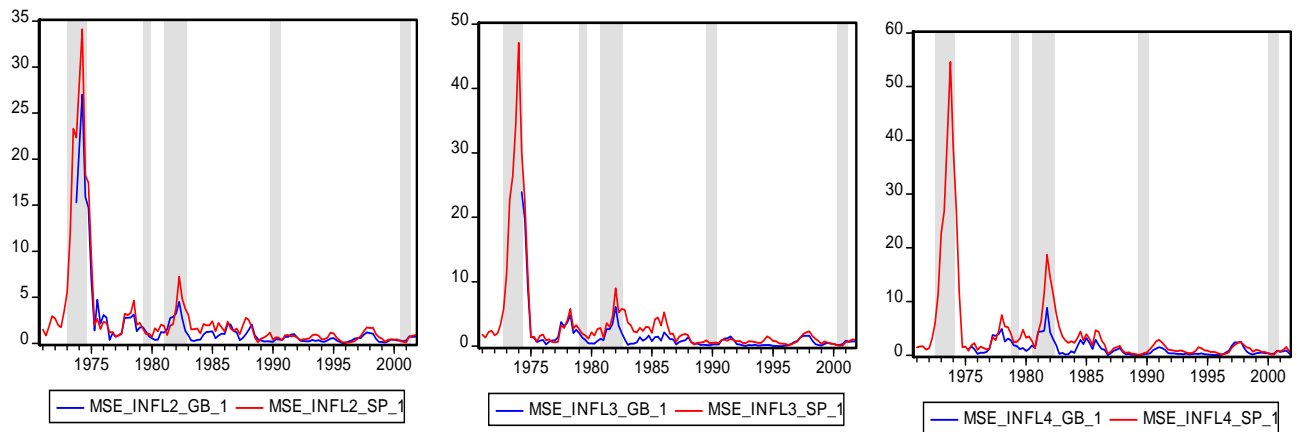
Figure 5: 1-Year Rolling MSE (Inflation)
