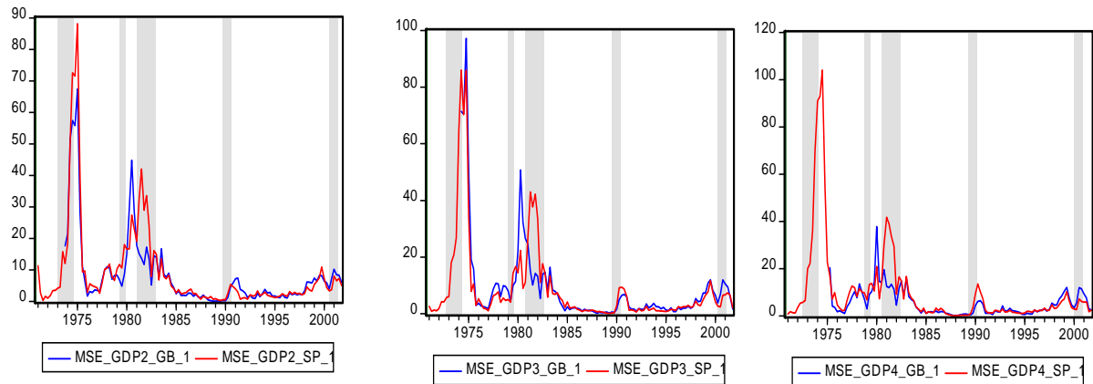
Figure 1: 1-Year Rolling MSE (GDP Growth)
