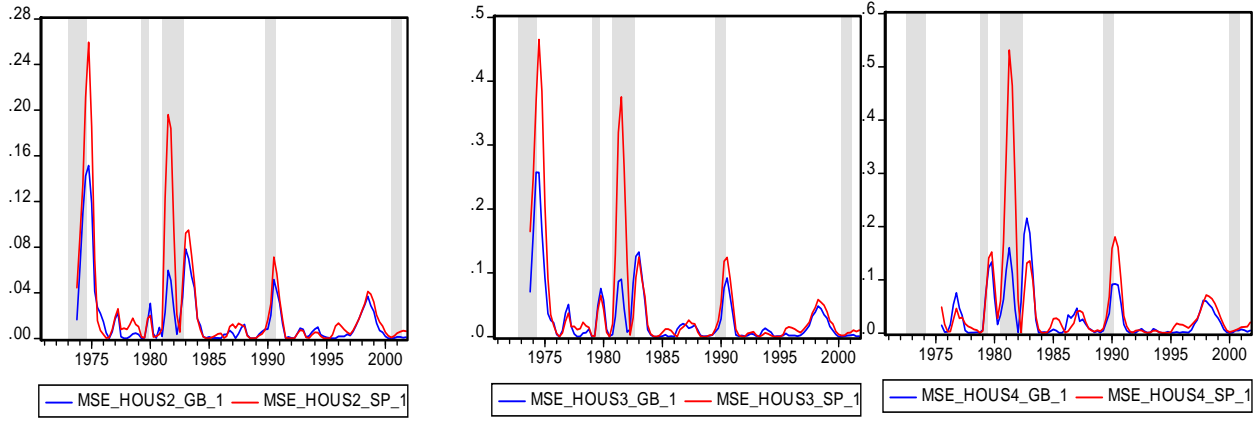
Figure 3: 1-Year Rolling MSE (Housing Starts)
