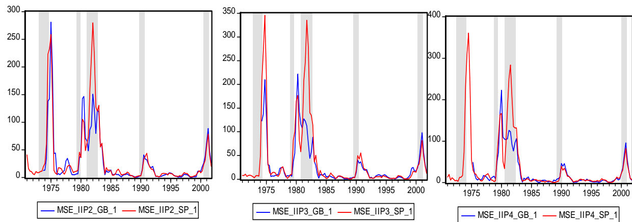
Figure 2: 1-Year Rolling MSE (Industrial Production)
