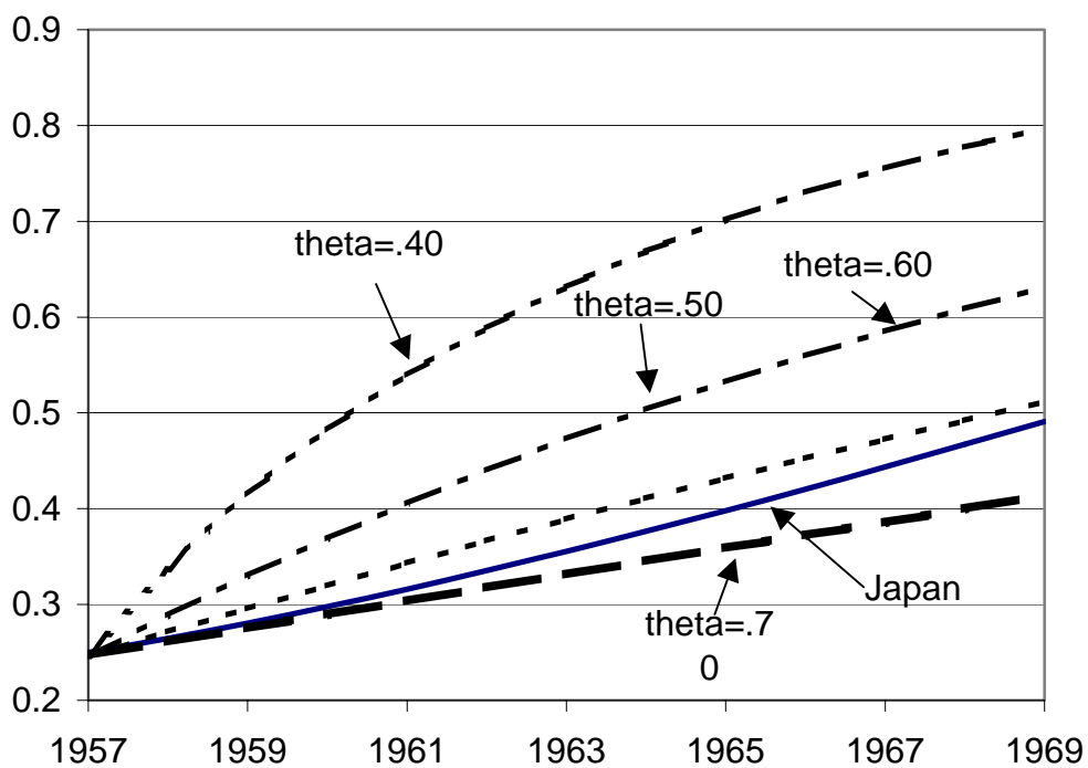
Figure 11: Growth Miracles
